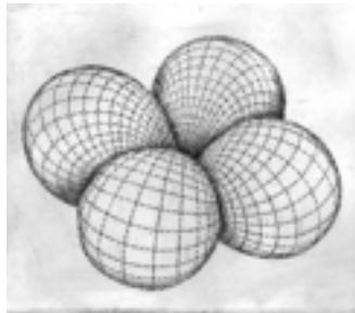
Fig. 24. Sievert's surface
