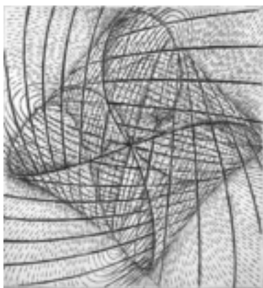
Fig. 19 Apéry model
